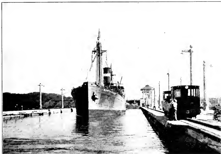
PANAMA CANAL: at the Ninafiores Locks, looking north, showing S. S. Santa Clara in lower west chamber, ready for water to be lowered to sea level.
